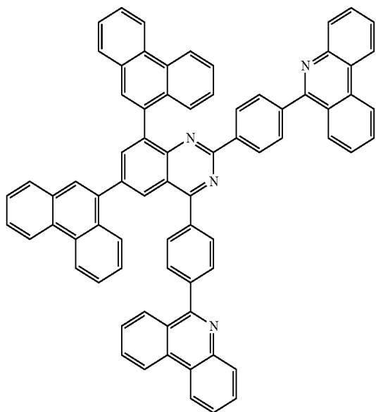
[Chemical Formula A-42]
