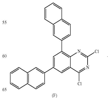
[Reaction Scheme 8]
