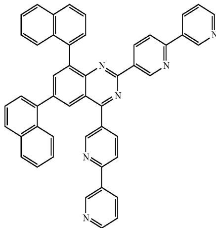
[Chemical Formula A-130]
