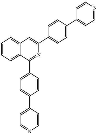
[Chemical Formula B-6]
