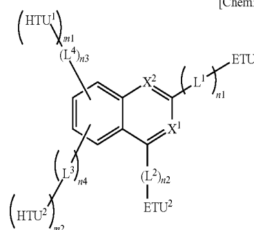
[Chemical Formula 2]
