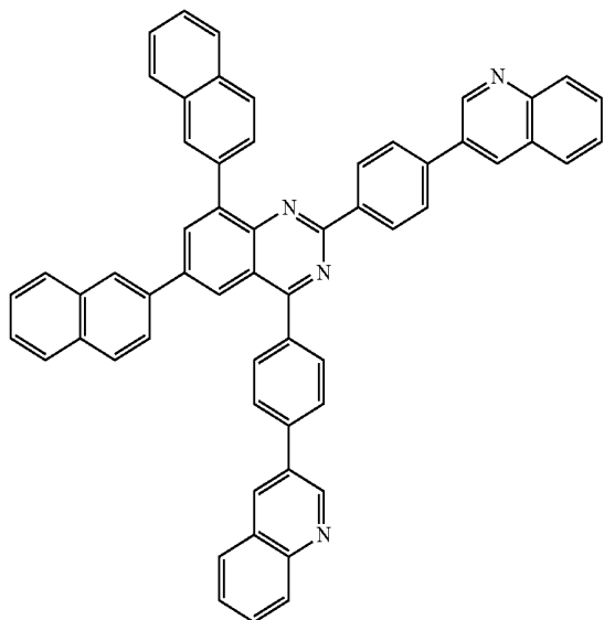
[Chemical Formula A-5]
