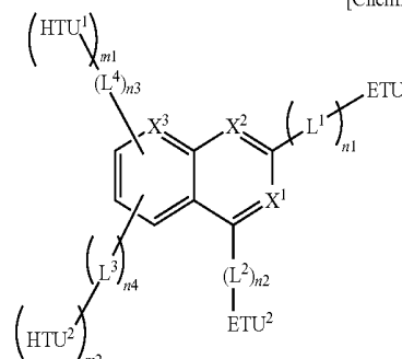
[Chemical Formula 1]
