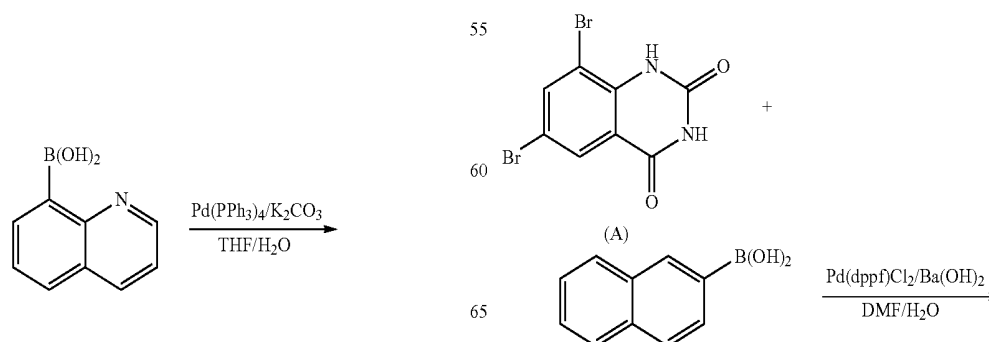
[Reaction Scheme 7]
