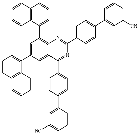
[Chemical Formula A-119]
