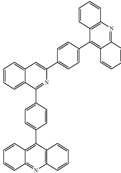
[Chemical Formula B-11]
