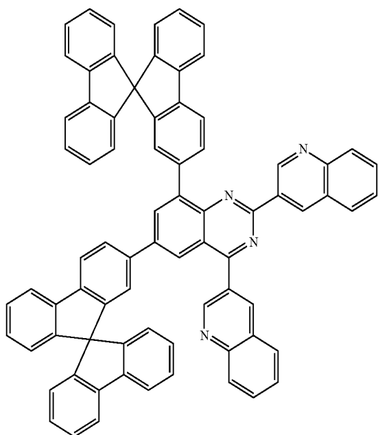
[Chemical Formula A-1]
