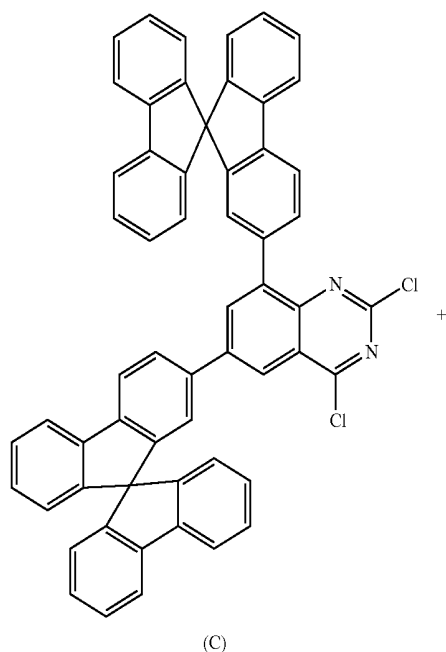
[Reaction Scheme 6]
