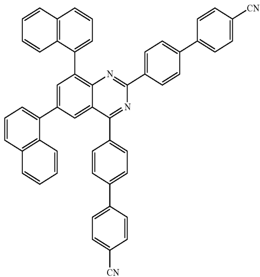
[Chemical Formula A-117]
