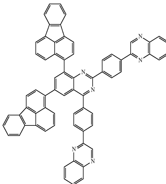
[Chemical Formula A-331]
